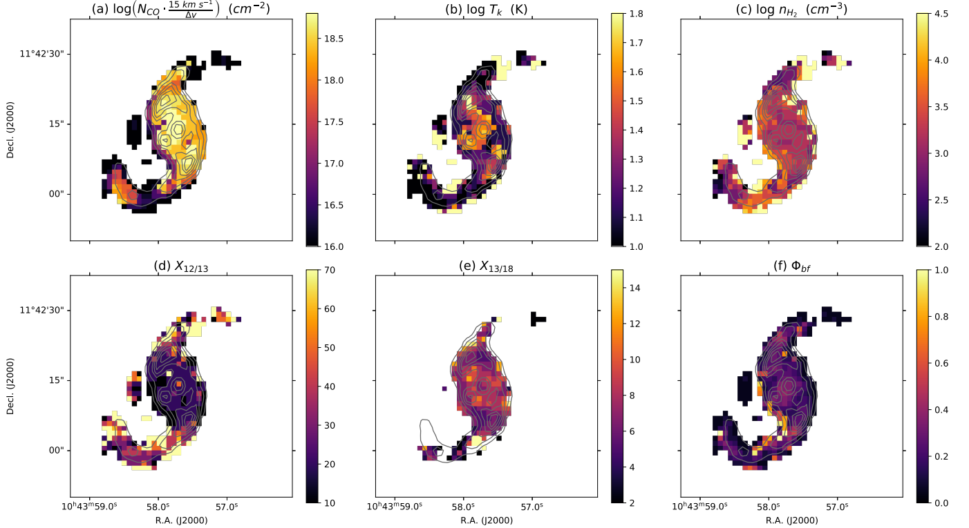
Figure 8. Maps of the 1DMax physical conditions derived from the one-component model. Panel (a) shows \log(N_{CO}) assuming a constant line width of 15 \text{ km s}^{-1} over the whole region. Contours represent the CO 2-1 emission shown in Figure 1b. A 1\sigma mask of the C 18 O 2-1 image is applied to (e). These results show that N_{CO} is higher in the center, T_k is higher near the nucleus and the contact points, and n_{H_2} is overall \sim 2 \times 10^3 \text{ cm}^{-3} . The X_{12/13} and X_{13/18} abundances are found to be consistent with those in the center of Milky Way.
