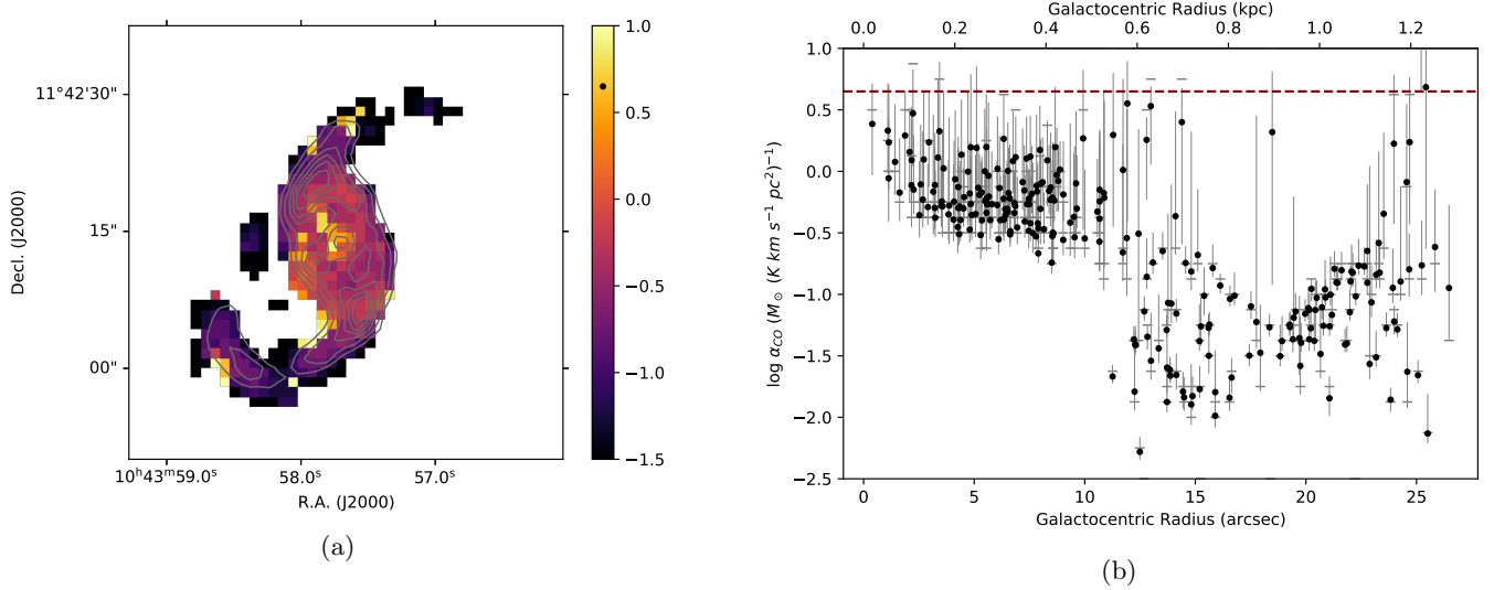
Figure 11. (a) 1DMax \log(\alpha_{\text{CO}}) map in units of \text{M}_{\odot} (\text{K km s}^{-1} \text{pc}^2)^{-1} . (b) Relation between the median/1DMax \alpha_{\text{CO}} and galactocentric radius, both derived from the two-component model using the marginalized \alpha_{\text{CO}} likelihoods. See the caption of Figure 10 for more information. The spatial variation of \alpha_{\text{CO}} and the values in the arms are similar to that derived from the one-component model, while the values in the center are a factor of 2–3 lower.
