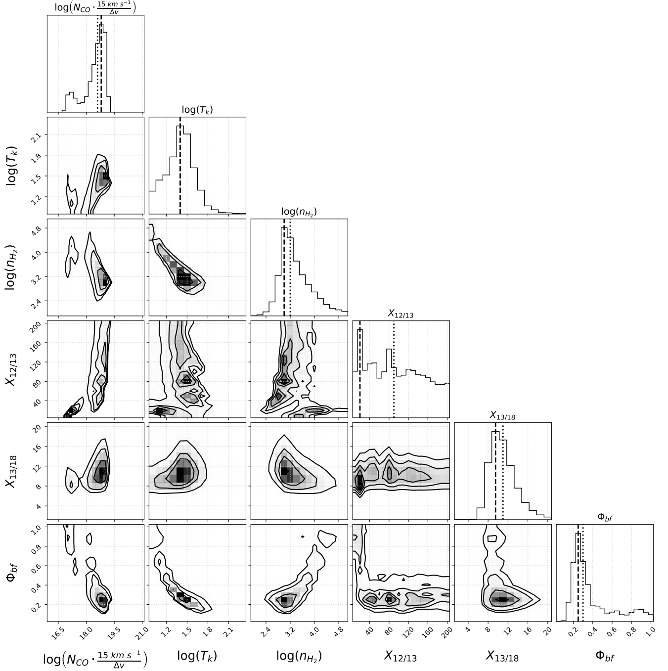
Figure 6. Marginalized 1D and 2D likelihood distributions of a faint pixel at (R.A., Decl.) = ( 10^{\text{h}}43^{\text{h}}57^{\text{m}}.8 , 11^{\circ}42'15''.5 ) in the gap region between the ring and the nucleus. See the caption of Figure 5 for more information.
