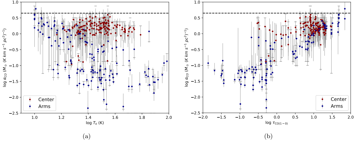
Figure 17. Relation between the median/1DMax \alpha_{\text{CO}} and (a) the median kinetic temperatures or (b) CO optical depths determined by the 1DMax physical conditions, both derived from the one-component modeling. The red/blue dots represent the median \alpha_{\text{CO}} in the center/arms, and the gray horizontal lines indicate the 1DMax \alpha_{\text{CO}} solutions. The 16th–84th percentile values of \alpha_{\text{CO}} are shown by the vertical lines. The dashed lines mark the Galactic \alpha_{\text{CO}} value. There is no signs of correlation between \alpha_{\text{CO}} and T_k , while \alpha_{\text{CO}} and \tau_{\text{CO}(1-0)} potentially shows a positive correlation.
