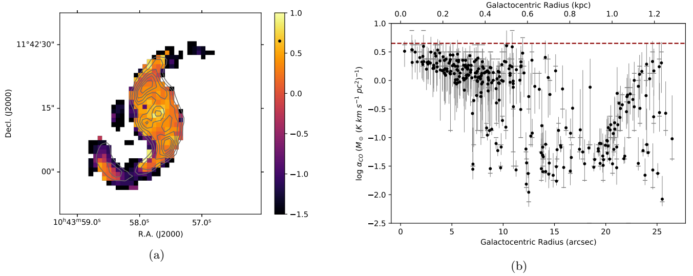
Figure 10. (a) 1DMax \log(\alpha_{\text{CO}}) map in units of \text{M}_{\odot} (\text{K km s}^{-1} \text{pc}^2)^{-1} ; the contours represent the CO 1–0 emission and the black dot on the color bar indicates the Galactic average value of \alpha_{\text{CO}} \sim 4.4 \text{ M}_{\odot} (\text{K km s}^{-1} \text{pc}^2)^{-1} . (b) Relation between the median \alpha_{\text{CO}} (black dots) and galactocentric radius, both derived from the one-component model using the marginalized \alpha_{\text{CO}} likelihoods; the gray horizontal lines represent the 1DMax \alpha_{\text{CO}} and the vertical lines show the 1\sigma ranges (16th–84th percentiles); the red dashed line shows the Galactic disk average value of \alpha_{\text{CO}} \sim 4.4 \text{ M}_{\odot} (\text{K km s}^{-1} \text{pc}^2)^{-1} . In the center, the median and 1DMax \alpha_{\text{CO}} values are only slightly below the Galactic disk average, and decrease slowly from the nucleus to the ring. Beyond a galactocentric radius of \sim 10'' , \alpha_{\text{CO}} drops significantly to a value that is approximately an order of magnitude lower than the Galactic disk average.
