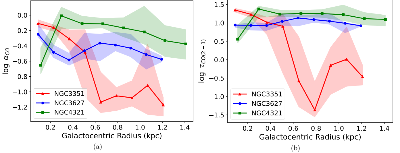
Figure 13. Medians of the modeled (a) \alpha_{\text{CO}} in units of \text{M}_{\odot} (\text{K km s}^{-1} \text{pc}^2)^{-1} and (b) line center \tau_{\text{CO}(2-1)} within \sim 100 pc galactocentric radii bins in the centers of NGC 3351 (red), NGC 3627 (blue), and NGC 4321 (green). Shaded areas span the 25th and 75th percentile ranges. All regions show \alpha_{\text{CO}} at least a factor of four lower than the Galactic value of \log(\alpha_{\text{CO}}) = 0.64 . The radial trend of \alpha_{\text{CO}} is mostly consistent with that of \tau_{\text{CO}(2-1)} in all three galaxy centers except in NGC 3627's nucleus.
