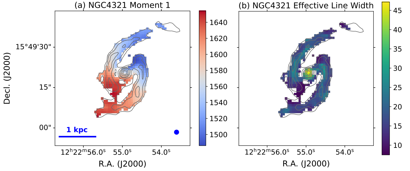
Figure 23. Maps of the CO 2-1 (a) moment 1 and (b) effective line width for NGC 4321, both in units of km s -1 .
